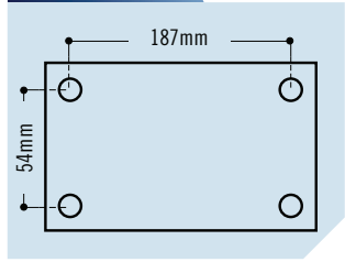
BOLT PATTERN
