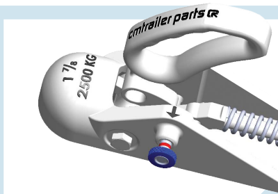
Handle up Red ring visible, Securalok safety lock pin not engaged
