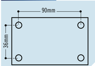
BOLT PATTERN
